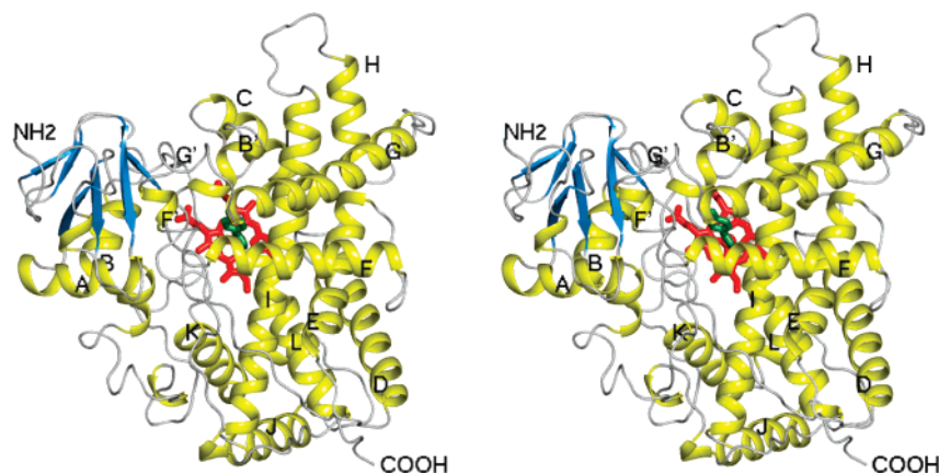
FIGURE 3: Divergent stereoview of the 2B4/1-CPI complex (molecule A). Helices and strands are colored yellow and blue, respectively. The termini and major helices are labeled. Heme and 1-CPI are shown as red and forest sticks, respectively.
