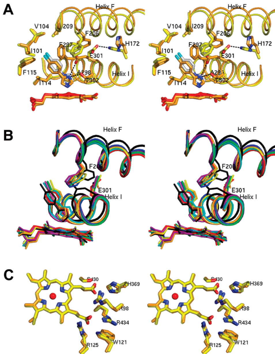
FIGURE 5: Divergent stereoviews for superposition of the 2B4/1-CPI and 2B4/4-CPI structures. (A) The 2B4/4-CPI structure superposed onto the 2B4/1-CPI (molecule A). Side chains of residues within a generous 5 Å contact distance from the ligands are shown as sticks and colored by elements (orange/yellow carbon in 2B4/4-CPI or 2B4/1-CPI, red oxygen, blue nitrogen, and cyan chlorine). The carbon atoms of 1-CPI are colored gray. Heme is shown as red (2B4/1-CPI) or orange (2B4/4-CPI) sticks. Helices F and I are labeled. (B) Overlay of 2B4/4-CPI and 7 molecules of 2B4/1-CPI in the asymmetric unit. The 2B4/4-CPI structure is colored black. The seven molecules of 2B4/1-CPI are colored red, orange, yellow, green, cyan, blue, and purple, respectively. (C) Heme coordination in 2B4/1-CPI (molecule A) and 2B4/4-CPI. Heme and side chains of residues involved in coordination of heme propionates are shown as sticks and colored by elements (yellow carbon, red oxygen, and blue nitrogen) in 2B4/1-CPI. These residues in the 2B4/4-CPI structure are also shown, and their carbon atoms are colored orange. The iron is displayed as a red sphere.
