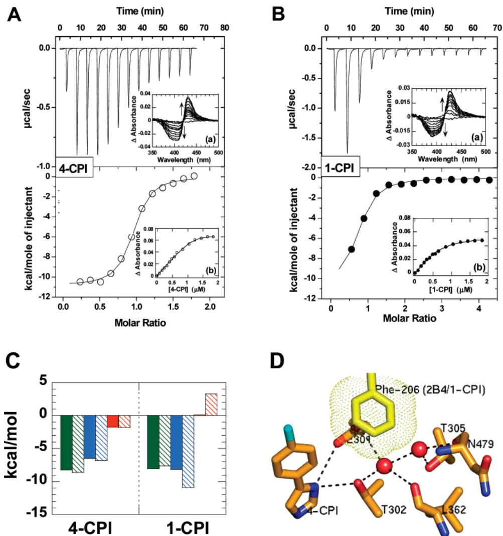
FIGURE 6: ITC and spectral studies of 4-CPI (A) and 1-CPI (B) binding to the F206A mutant. The upper panels show the enthalpy changes, and the lower panels are the resulting integrated enthalpy data fit to a single binding site model. The equilibrium difference spectra data are shown in the upper panels (inset a). The spectral data were fit to the “tight binding” equation, yielding the binding curve shown in the lower panels (inset b). (C) Thermodynamic signatures of 4-CPI and 1-CPI binding to 2B4dH(H226Y) (10) (solid bars) and F206A (hatched bars) are compared. Binding free energy ( \Delta G ), green; change in enthalpy ( \Delta H ), blue; change in entropy ( -T\Delta S ), red. (D) The network of 8 hydrogen bonds in the 2B4/4-CPI structure. 4-CPI, Leu-362, Asn-479, and the side chains of Glu-301, Thr-302, and Thr-305 are shown as sticks and colored by elements (orange carbon, red oxygen, blue nitrogen, and cyan chlorine). Two waters are shown as red spheres. Hydrogen bonds are indicated by dashed lines. This network of hydrogen bonds must be diminished in the 2B4/1-CPI complex, because the new position of the Phe-206 side chain, which is shown as yellow sticks, requires the displacement of two water molecules. The van der Waals radius of the Phe-206 side chain is indicated by small dots.
