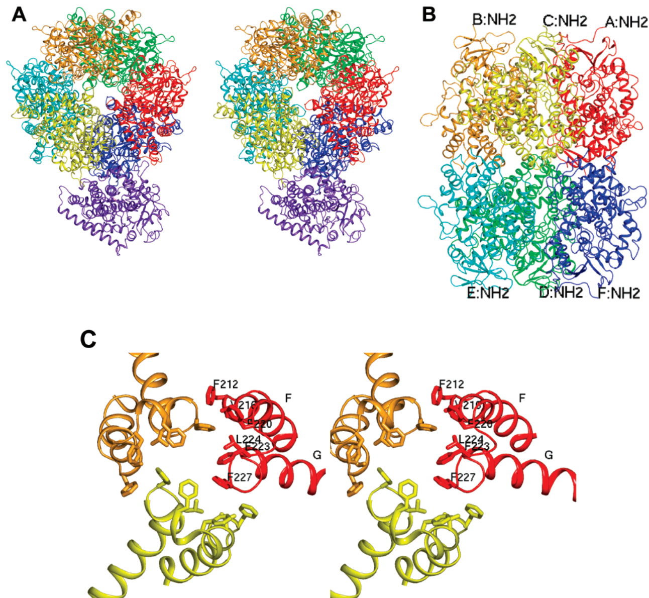
FIGURE 2: (A) Divergent stereoview of the seven copies of 2B4/1-CPI in the asymmetric unit. The seven molecules are shown as ribbon diagrams and colored red (molecule A), orange (B), yellow (C), green (D), cyan (E), blue (F), and purple (G), respectively. The view is along the 3-fold axis of the hexamer. (B) Side view of the hexamer. The color scheme is the same as in (A), and N-termini are indicated. (C) Divergent stereoview of hydrophobic interactions around the 3-fold axis of trimer ABC. Molecules A, B, and C are colored red, orange, yellow, respectively. The side chains of F212, V216, F220, F223, L224, and F227 are shown as sticks. These residues and helices F and G are labeled in molecule A.
